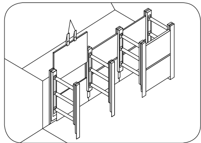
Figure 7: Plate lining system.
