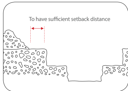
Figure 2: Benching control.
